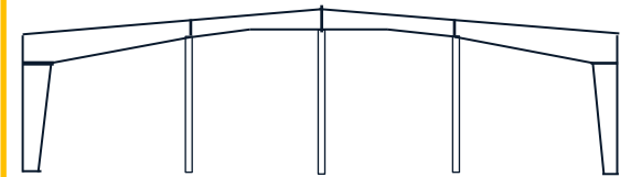
MULTI SPAN (TYPE 3)
